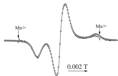
Figure 4 EPR spectrum of the radical in MBBA at 77 K (line) and the simulation result of this spectrum (circles).
