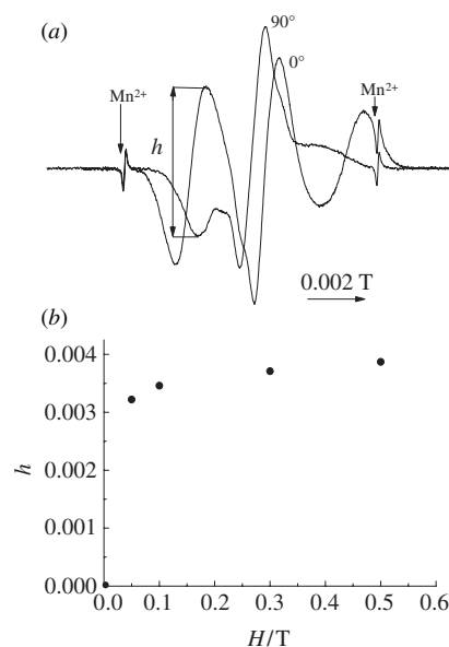
Figure 5 (a) EPR spectra of radical in aligned MBBA recorded at 0^\circ and 90^\circ between the director of the liquid crystal and the magnetic field vector; (b) the dependence of h on magnetic field strength; h is normalised over the number of paramagnetic particles.
